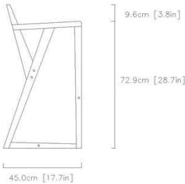
04 / FULL-SIZE TECHNICAL PROFILE & DIMENSIONS
