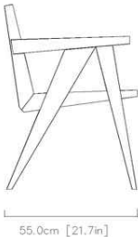
04 / FULL-SIZE TECHNICAL PROFILE & DIMENSIONS
