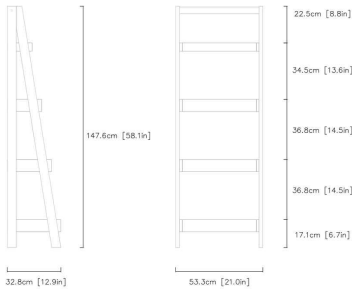
04 / FULL-SIZE TECHNICAL PROFILE & DIMENSIONS
