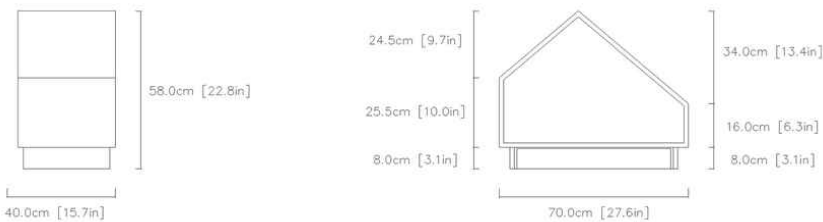
04 / FULL-SIZE TECHNICAL PROFILE & DIMENSIONS
