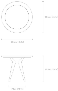
04 / FULL-SIZE TECHNICAL PROFILE & DIMENSIONS
