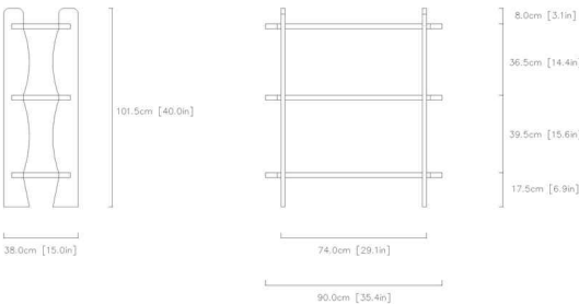
04 / FULL-SIZE TECHNICAL PROFILE & DIMENSIONS
