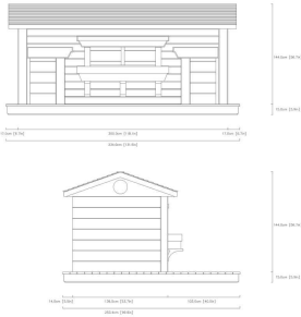
04 / FULL-SIZE TECHNICAL PROFILE & DIMENSIONS
