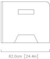
04 / FULL-SIZE TECHNICAL PROFILE & DIMENSIONS
