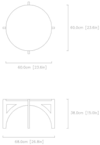
04 / FULL-SIZE TECHNICAL PROFILE & DIMENSIONS
