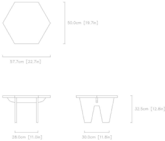
04 / FULL-SIZE TECHNICAL PROFILE & DIMENSIONS
