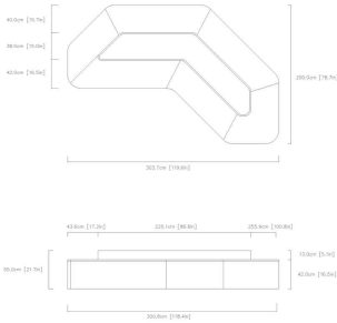
04 / FULL-SIZE TECHNICAL PROFILE & DIMENSIONS
