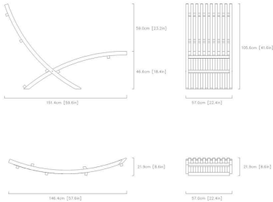
04 / FULL-SIZE TECHNICAL PROFILE & DIMENSIONS
