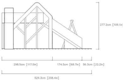
04 / FULL-SIZE TECHNICAL PROFILE & DIMENSIONS
