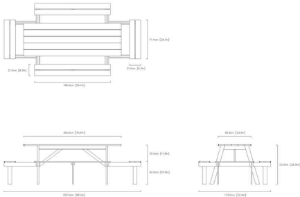
04 / FULL-SIZE TECHNICAL PROFILE & DIMENSIONS
