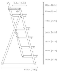
04 / FULL-SIZE TECHNICAL PROFILE & DIMENSIONS
