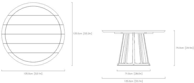
04 / FULL-SIZE TECHNICAL PROFILE & DIMENSIONS
