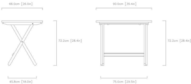
04 / FULL-SIZE TECHNICAL PROFILE & DIMENSIONS
