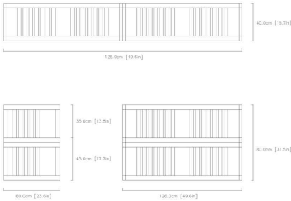
04 / FULL-SIZE TECHNICAL PROFILE & DIMENSIONS
