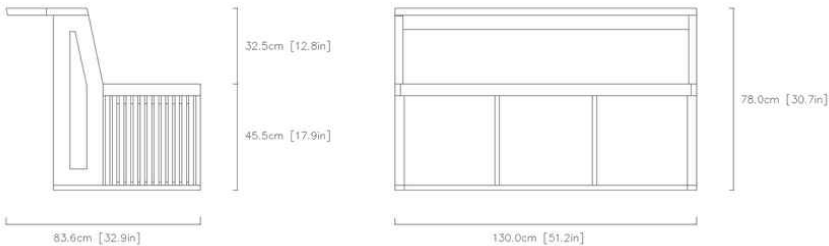
04 / FULL-SIZE TECHNICAL PROFILE & DIMENSIONS
