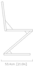
04 / FULL-SIZE TECHNICAL PROFILE & DIMENSIONS
