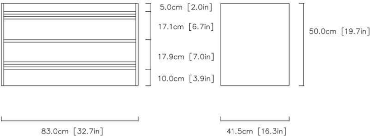
04 / FULL-SIZE TECHNICAL PROFILE & DIMENSIONS
