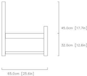
04 / FULL-SIZE TECHNICAL PROFILE & DIMENSIONS
