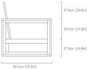
04 / FULL-SIZE TECHNICAL PROFILE & DIMENSIONS
