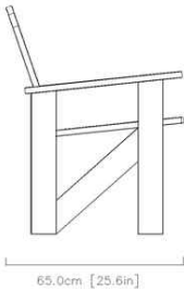
04 / FULL-SIZE TECHNICAL PROFILE & DIMENSIONS
