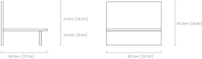
04 / FULL-SIZE TECHNICAL PROFILE & DIMENSIONS
