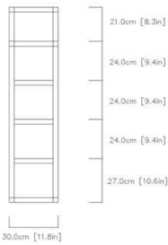
04 / FULL-SIZE TECHNICAL PROFILE & DIMENSIONS
