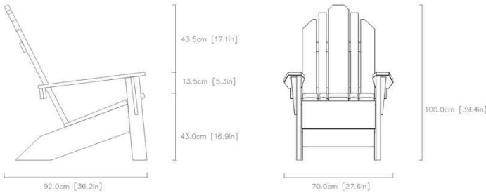
04 / FULL-SIZE TECHNICAL PROFILE & DIMENSIONS
