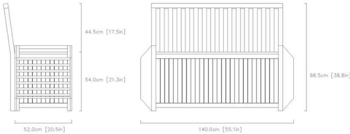
04 / FULL-SIZE TECHNICAL PROFILE & DIMENSIONS
