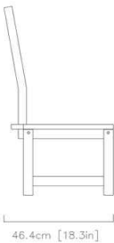
04 / FULL-SIZE TECHNICAL PROFILE & DIMENSIONS
