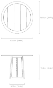
04 / FULL-SIZE TECHNICAL PROFILE & DIMENSIONS
