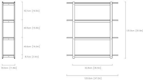
04 / FULL-SIZE TECHNICAL PROFILE & DIMENSIONS
