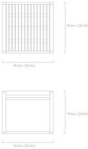
04 / FULL-SIZE TECHNICAL PROFILE & DIMENSIONS
