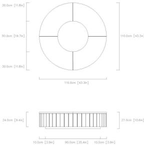
04 / FULL-SIZE TECHNICAL PROFILE & DIMENSIONS
