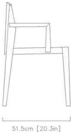
04 / FULL-SIZE TECHNICAL PROFILE & DIMENSIONS
