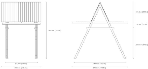
04 / FULL-SIZE TECHNICAL PROFILE & DIMENSIONS
