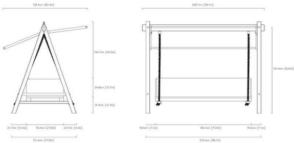
04 / FULL-SIZE TECHNICAL PROFILE & DIMENSIONS
