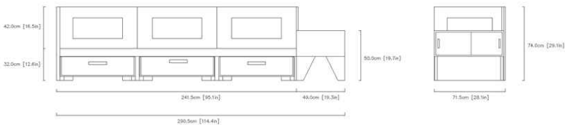
04 / FULL-SIZE TECHNICAL PROFILE & DIMENSIONS
