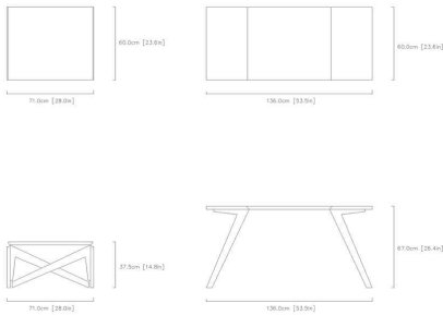
04 / FULL-SIZE TECHNICAL PROFILE & DIMENSIONS
