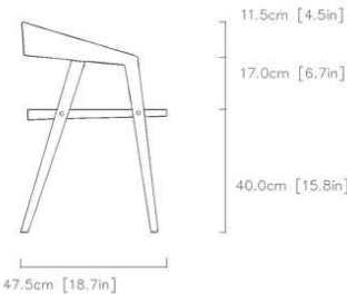
04 / FULL-SIZE TECHNICAL PROFILE & DIMENSIONS
