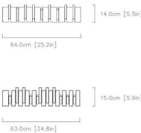
04 / FULL-SIZE TECHNICAL PROFILE & DIMENSIONS
