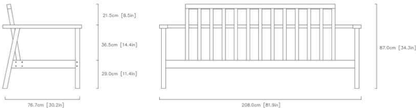
04 / FULL-SIZE TECHNICAL PROFILE & DIMENSIONS
