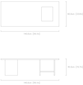
04 / FULL-SIZE TECHNICAL PROFILE & DIMENSIONS
