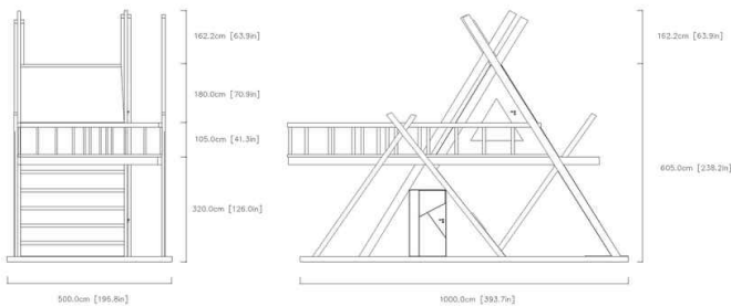
04 / FULL-SIZE TECHNICAL PROFILE & DIMENSIONS
